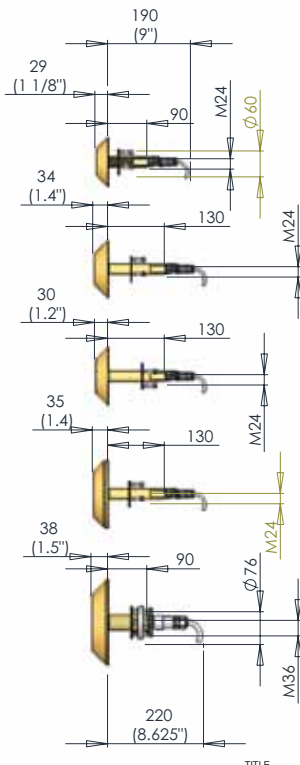
1010 THRU HULL
